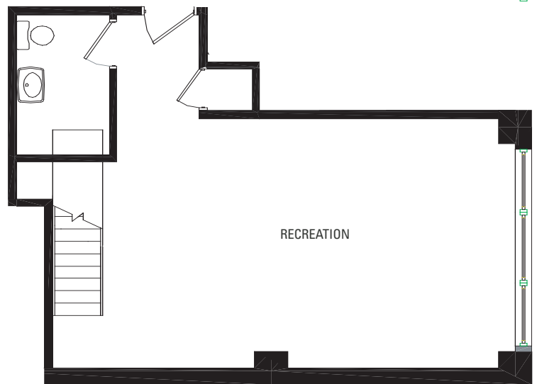
LOWER FLOOR
